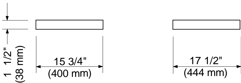
SCALE BASE
